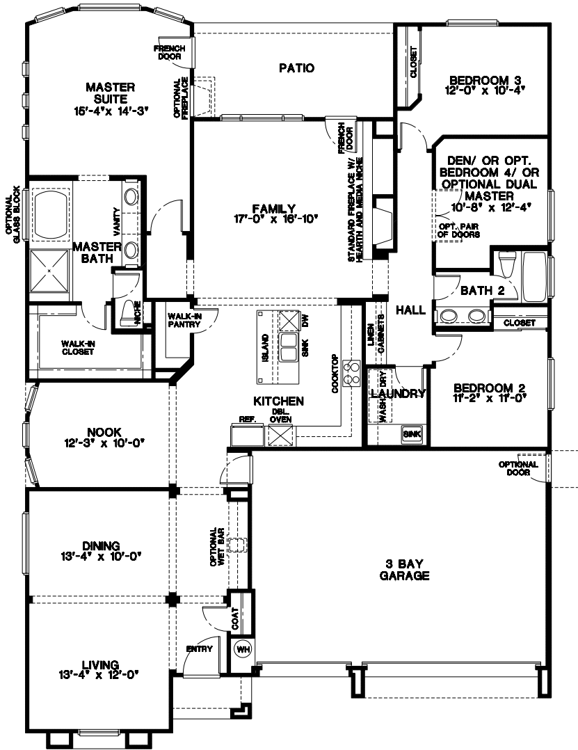
FLOOR PLAN
